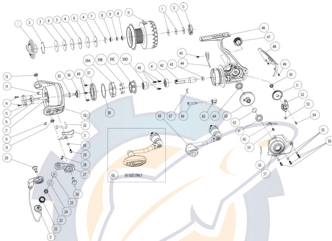
Quantum Catalyst Inshore CI50PTsB Spinning Reel Part List
